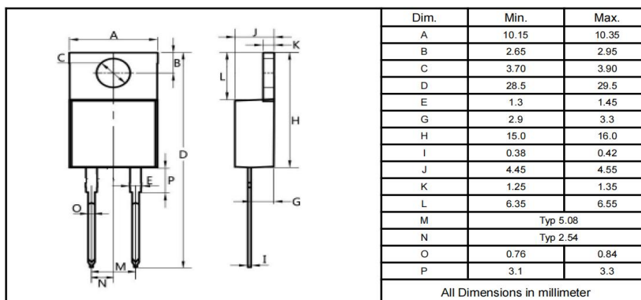
TO-220FAC
